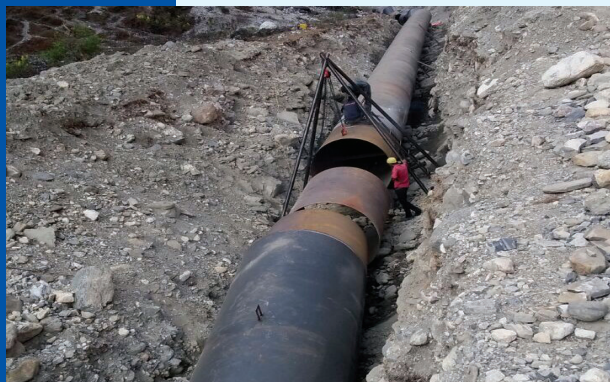
Pipe Alignment at Upper Naugarh
