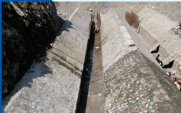
Desander under construction at Upper Naugarh
