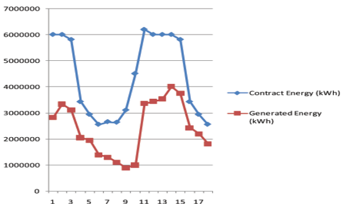
Naugarh Gad Small Hydroelectric Project (8.5 MW) Energy Generation
